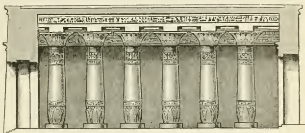
Section of Hall, Ramesseum, Thebes.
