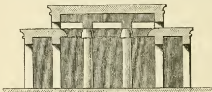
Section of smaller Pillared Hall, Great Temple, Karnak.
