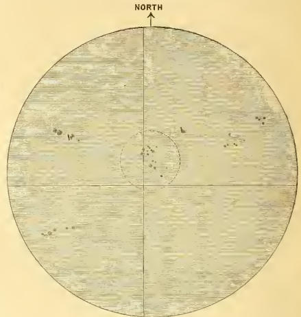
Tracing from sun negative taken at Dehra Observatory, Great Trigonometrical Survey of India. Latitude 30^{\circ} 16' 29'' N.; Longitude 78^{\circ} 5' 49'' E. Height above sea 2232 feet, on July 25, 1881, at 4.47 p.m. local apparent time. Spots visible in previous negative taken on the same day at 3.58 p.m. are coloured black; and the new spots which appeared between 4 and 5 p.m. are surrounded by a dotted circle.
