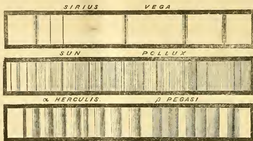
FIG. 27.—Three chief types of stellar spectra.
