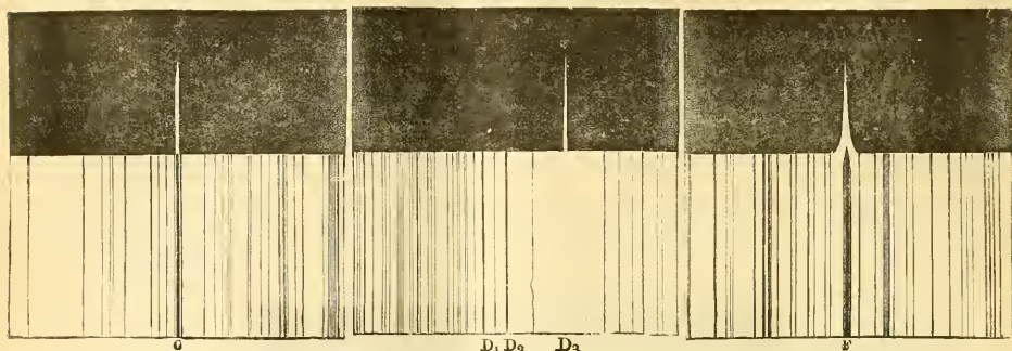
FIG. 10.—Line C (red), with radial slit.
