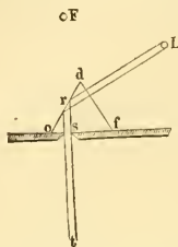
FIG. 5.—Path of light through comparison prism. d , f , o , prism, L , light source; r , point of reflection; s , slit; F , light source in front of slit.
