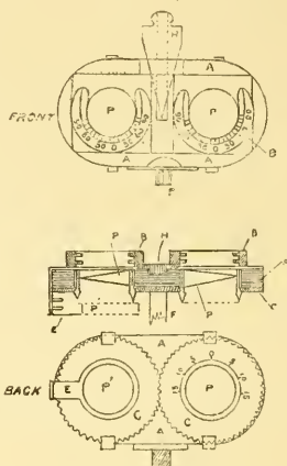
A, main frame carried by F, graduated rod; C, rotating frame carrying P, P, prisms; E, frame carrying F, third prism; H, wedge to separate B B frames for lenses.
