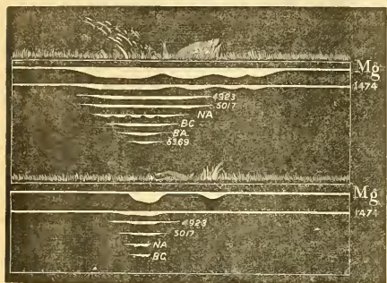
FIG. 23.—Chromosphere with jets (Tacchini).
