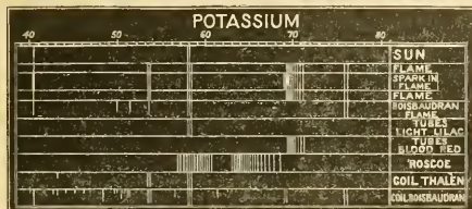
FIG. 49.—Spectra of potassium obtained under different conditions.
