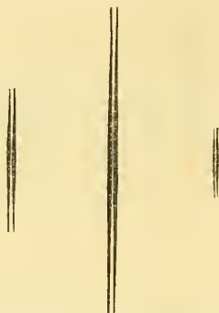
FIG. 25.—Spectrum of sodium, showing the long and short lines.
