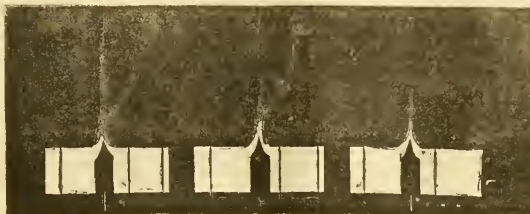
FIG. 16.—Alterations of wave-length in prominences. The dots show \frac{1}{100000000} mm.
