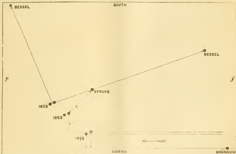
FIG. 1.—61 Cygni and parallax comparison stars.
