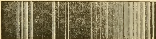
FIG. 30.—Carbon flutings, contrasted with the line-spectra of calcium, iron, aluminium, and other impurities of the poles.
