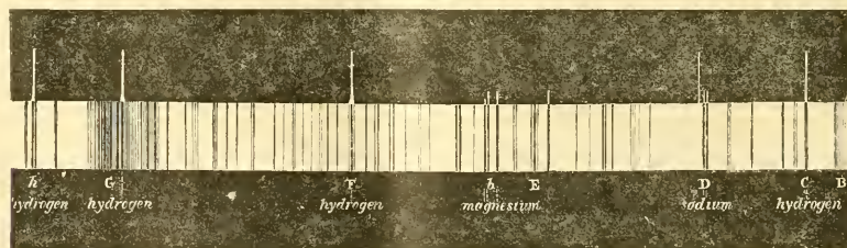
FIG. 13.—Spectrum of the sun's photosphere (below) and chromosphere (above).
