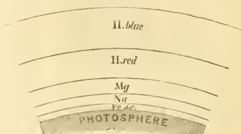
FIG. 21.—Stratification of the solar atmosphere.
