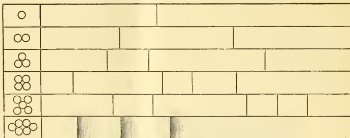
FIG. 46.—Diagram showing how the evolution of chemical forms may be indicated by their spectra.
