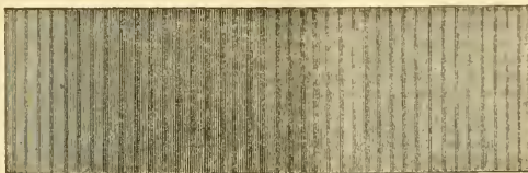
FIG. 29.—Fluted spectrum of iodine.
