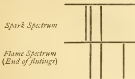
FIG. 42.—Flame and spark spectra of magnesium.
