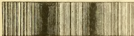
FIG. 2.—Copy of a photograph of the solar spectrum in the region of the thick calcium lines, by Lockyer.
