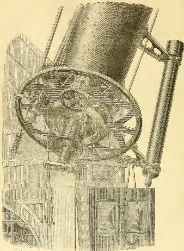
FIG. 2.—Eye-End and Breech-Piece of Telescope. A is the micrometer eye-piece; m, handles for working the focusing screw; c, eye-piece of finder telescope, 4 in. aperture; d, eye-piece of reader for reading right ascension and declination circles; e, handle for revolving same to point to various verniers; f, clamping handle in declination; g, slow motion handle in declination; h, clamping cords for right ascension; i, slow motion cord for right ascension; k, quick motion handle for right ascension and declination movements; l, flute key for position circle clamping; m, window through which glass position circle is viewed while illuminated from behind by beam of light from gas-lamp at end of declination axis; n, screw for slow motion in position angle; o, key for throwing into position a set of illuminators for "dark field" illumination of micrometer; p, handle for throwing into position an arm carrying one central mirror for "bright field" illumination of micrometer.
