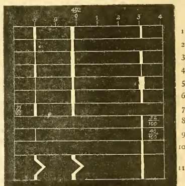
FIG. 41.— Behav. , &c., showing the behaviour of three iron lines under different conditions, solar and terrestrial. 1, solar spectrum; 2, arc; 3, quantity coil with jar; 4, quantity coil without jar; 5, intensity coil with jar; 6, intensity coil without jar; 7, spots observed at Kensington; 8, Prominences observed by Tacchini; 9, prominences observed by Young; 10, reversed in penumbra of spot observed on August 5, 1872, by Young; 11, motion indicated by change of refrangibility.
