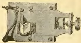
FIG. 4.—Steinheil's slit, showing reflecting prism.
