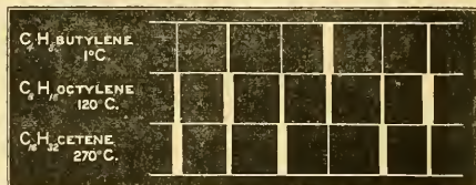
FIG. 47.—Hypo-theoretical spectra obtained on distilling at successively increasing temperatures a mixture of light and heavy hydrocarbons.
