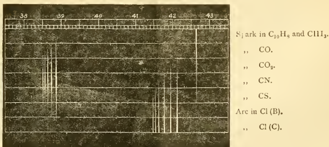
FIG. 45.—The photographed spectra of some carbon compounds.
