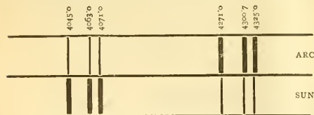
FIG. 40.—Anomalous reversals (iron) from a photograph.
