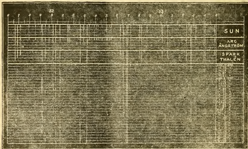
FIG. 5.—Portion of a large map showing the lines most affected in 100 sun-spots observed at South Kensington.
