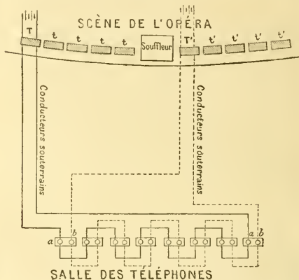
FIG. 2.—Connections between Opera and hearing-room.
