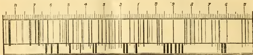
FIG. 34.—Spectrum of sun-spot observed at Greenwich.
