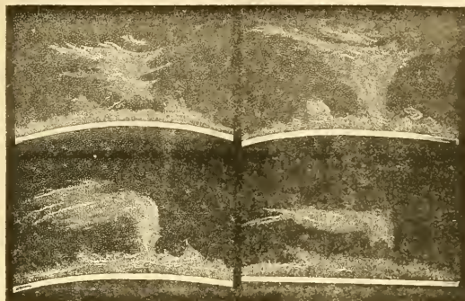
FIG. 14.—Solar prominences (Voog), showing lateral currents.
