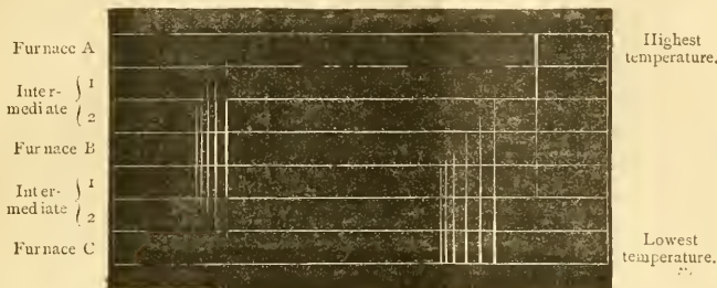
FIG. 44.—Diagram showing the action of three different temperatures on a hypothetical substance, assuming three stages of complete dissociation; and also of intermediate temperatures at which the vapours are only partially dissociated.
